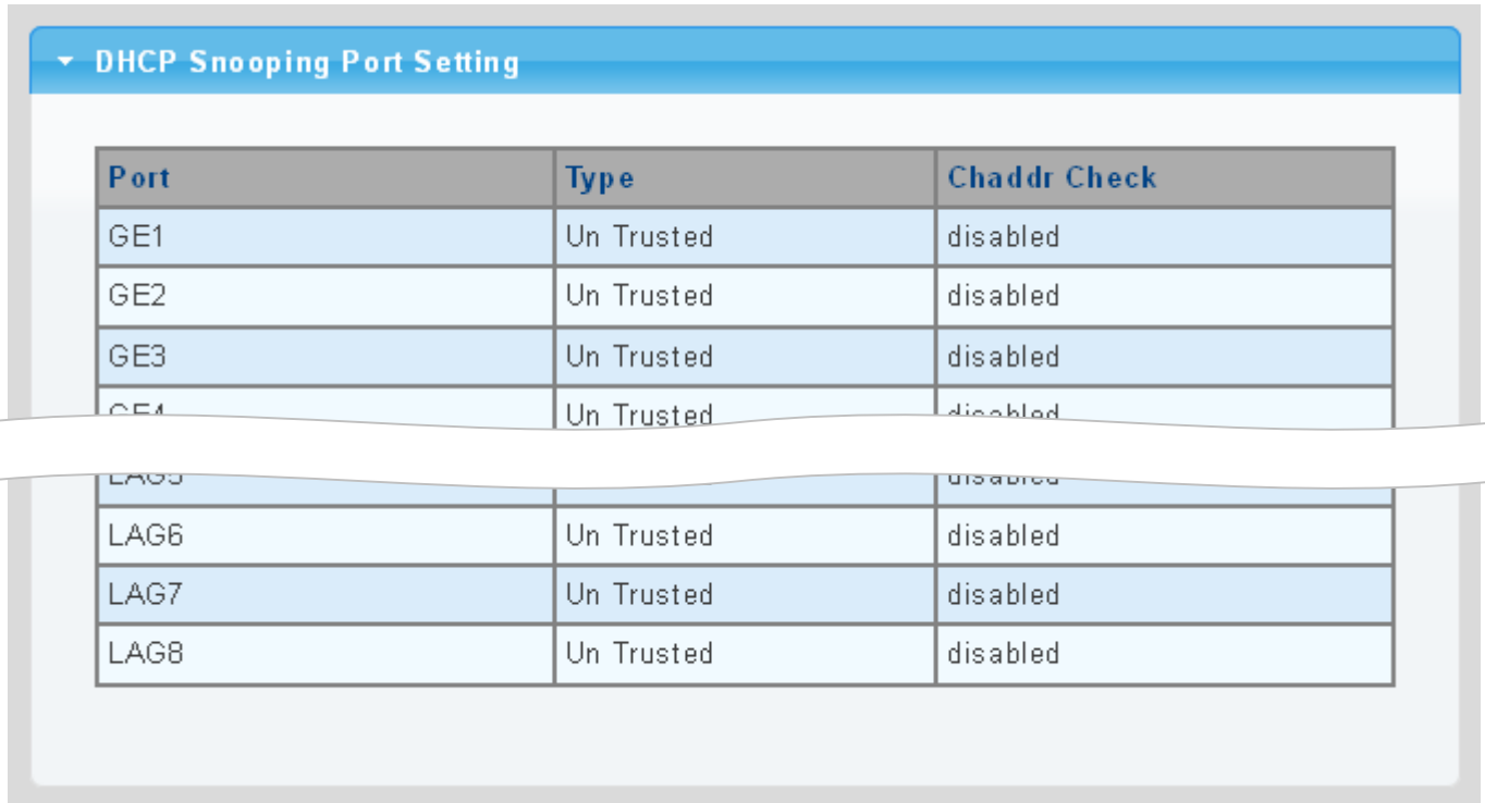
Figure 4-13-6-6: DHCP Snooping Port Setting Page Screenshot
