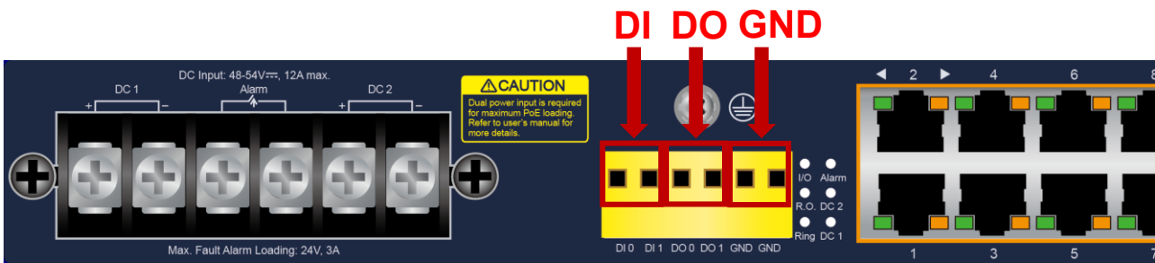
Figure 2-1-7-1b Wiring Digital Inputs/Outputs of IGS-R4215-24P4X
