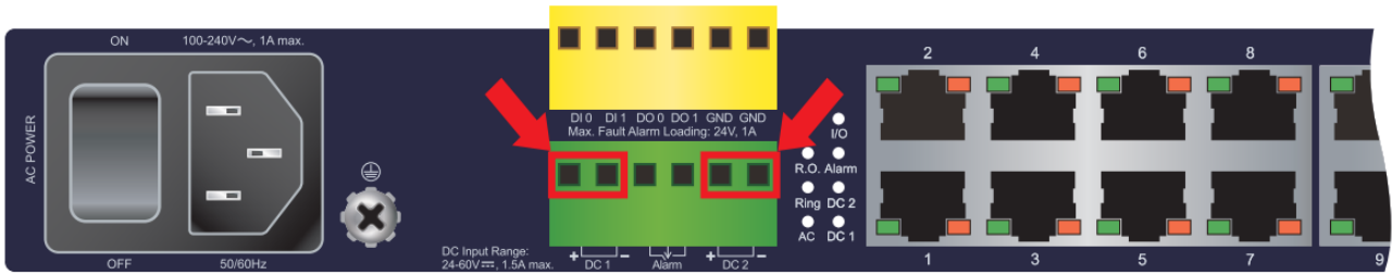
Figure 2-1-5-1: IGS-R4215-24T4X DC power input
