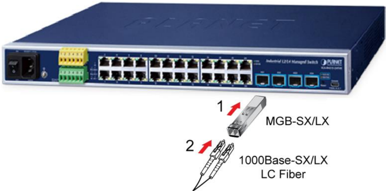
Figure 2-3-1-1: Plug in the SFP/SFP+ Transceiver
