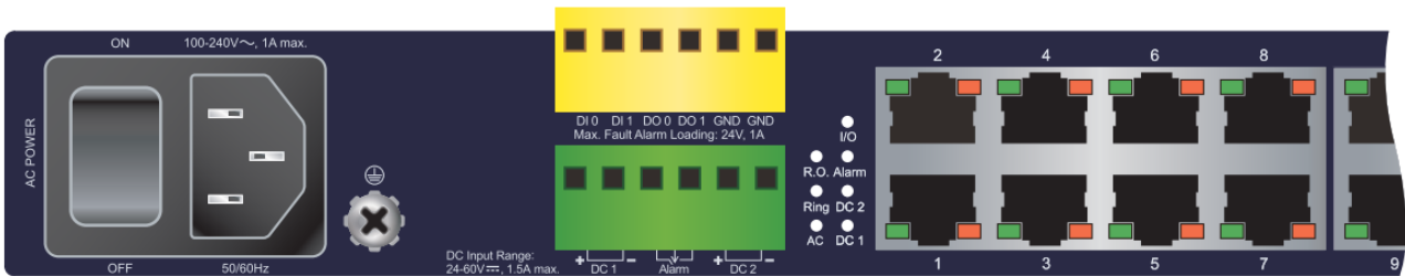
Figure 2-1-3-1a: IGS-R4215-24T4X LEDs on Front Panel
