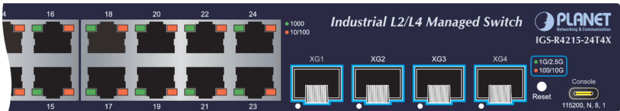
Figure 2-1-3-1b: IGS-R4215-24T4X LEDs on Front Panel
