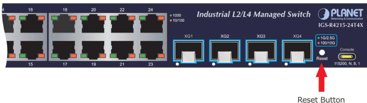
Figure 2-1-2-2a: Rest Button of IGS-R4215-24T4X
