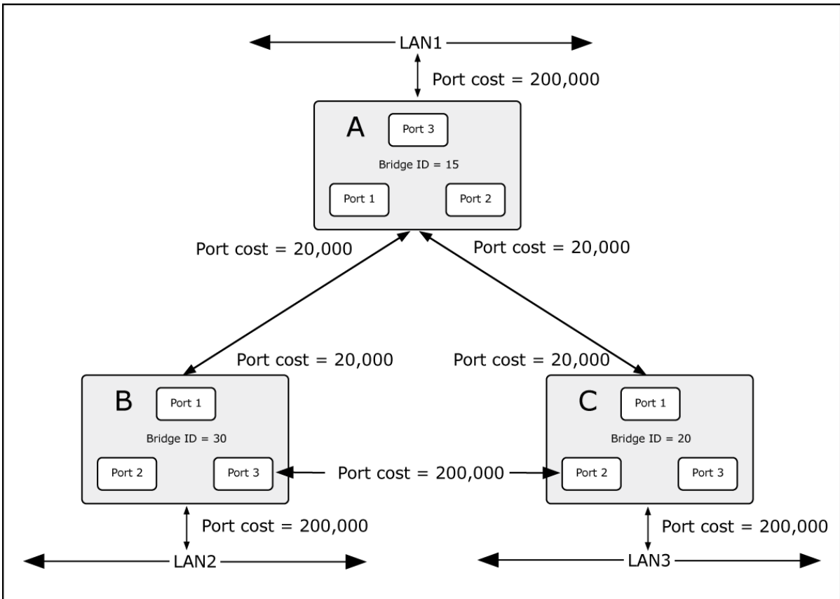
Figure 4-6-1-2: Before Applying the STA Rules
