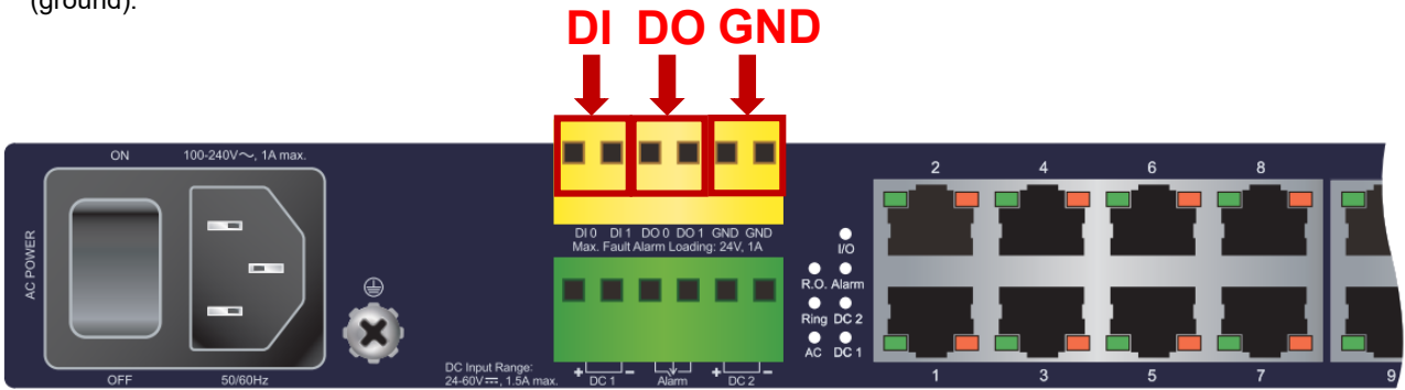
Figure 2-1-7-1a Wiring Digital Inputs/Outputs of IGS-R4215-24T4X
