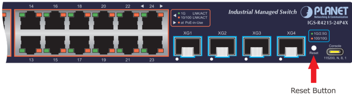
Figure 2-1-2-2b: Rest Button of IGS-R4215-24P4X
