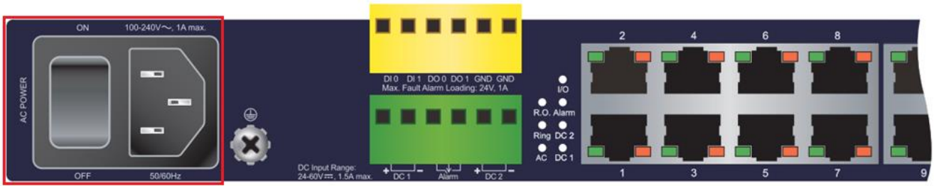
Figure 2-1-4-1: IGS-R4215-24T4X AC inlet power socket
