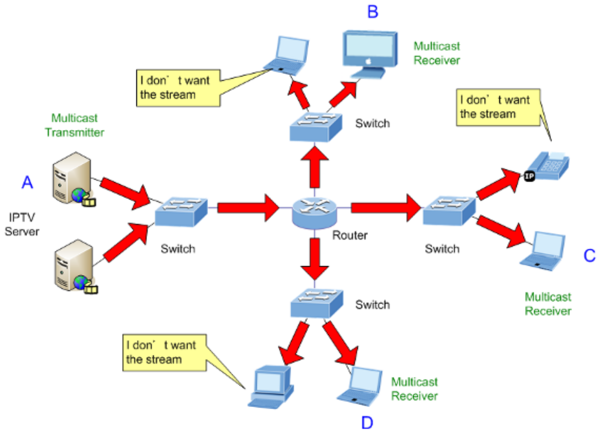
Figure 4-8-2: Multicast Flooding
