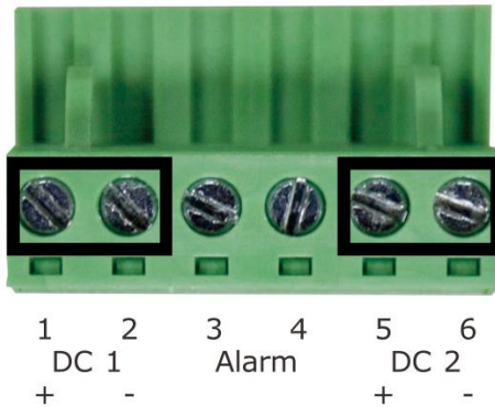
Figure 2-1-5-2 6-pin Terminal Block Power Wiring Input for IGS-R4215-24T4X
